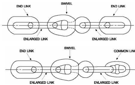
Typical Swivel Assemblies
